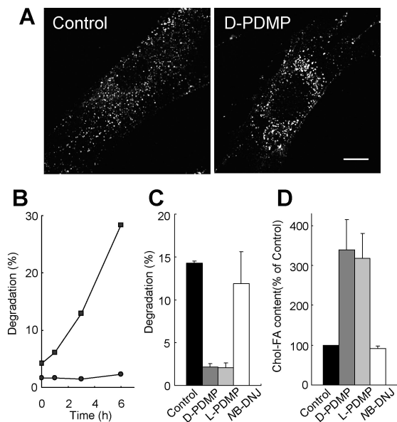
FIGURE 6: D-PDMP and L-PDMP but not NB-DNJ inhibit hydrolysis of [cholesteryl-4- ^{14} C] oleate-containing LDL. (A) Uptake of reconstituted LDL in the absence (control) and the presence of 10 \mu M D-PDMP (D-PDMP). Incorporation of BODIPY FL C12-containing LDL was measured as described in Materials and Methods. (B, C) Hydrolysis of [cholesteryl-4- ^{14} C] oleate-containing LDL was quantified as described in Materials and Methods. (B) Time course of degradation. Squares show the results in the absence of D-PDMP whereas circles indicate the degradation in the presence of 10 \mu M D-PDMP. (C) The effects of various drugs on the degradation of [cholesteryl-4- ^{14} C] oleate-containing LDL were measured after 6 h incubation. Control, without inhibitor; D-PDMP, 10 \mu M D-PDMP; L-PDMP, 10 \mu M L-PDMP; NB-DNJ, 500 \mu M NB-DNJ. Data are mean of triplicate experiments \pm SD. (D) Human skin fibroblasts were grown in the presence and absence of inhibitors for 3 days. Lipids were extracted and separated on TLC, and the content of cholesterol ester was measured as described in Materials and Methods. Control, without inhibitor; D-PDMP, 10 \mu M D-PDMP; L-PDMP, 10 \mu M L-PDMP; NB-DNJ, 500 \mu M NB-DNJ. Data are mean of triplicate experiments \pm SD.
